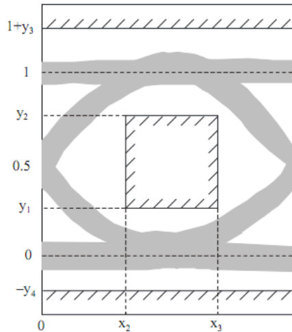
Figure 1 XGSPON Transmitter Eye Mask Definitions
